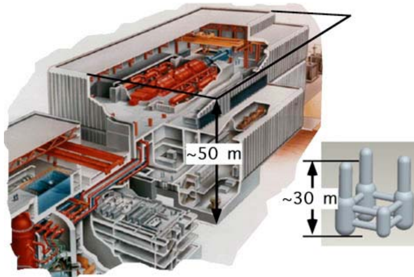
Fig. 1 Size comparison between the power conversion units of a very-high-temperature, 1300 MW(e) MCGC, and the 1380 MW(e) turbine building of the Advanced Boiling Water Reactor (courtesy GE Nuclear Energy). The MCGC turbine building will also require space for a crane, turbine lay-down space, cooling water circulation equipment, switchgear and high-pressure gas storage. The MCGC requires 1100 MW(t) of cooling water capacity, compared to 2800 MW(t) for the steam cycle.
