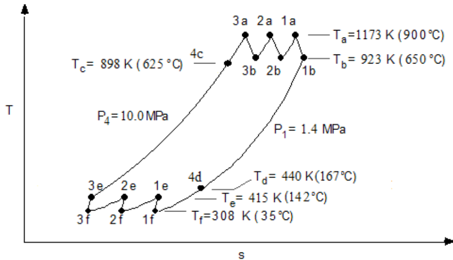
Fig. 6 Temperature-entropy diagram for the MCGC very-high-temperature reference case.
